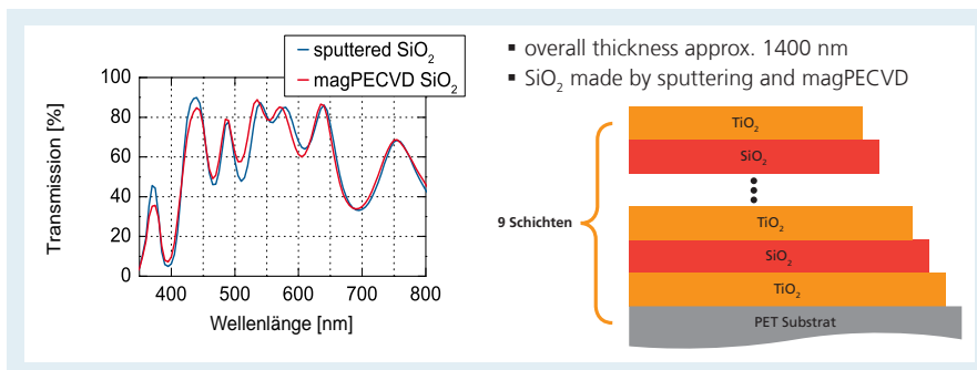
Dielectric solar control layer stacks
